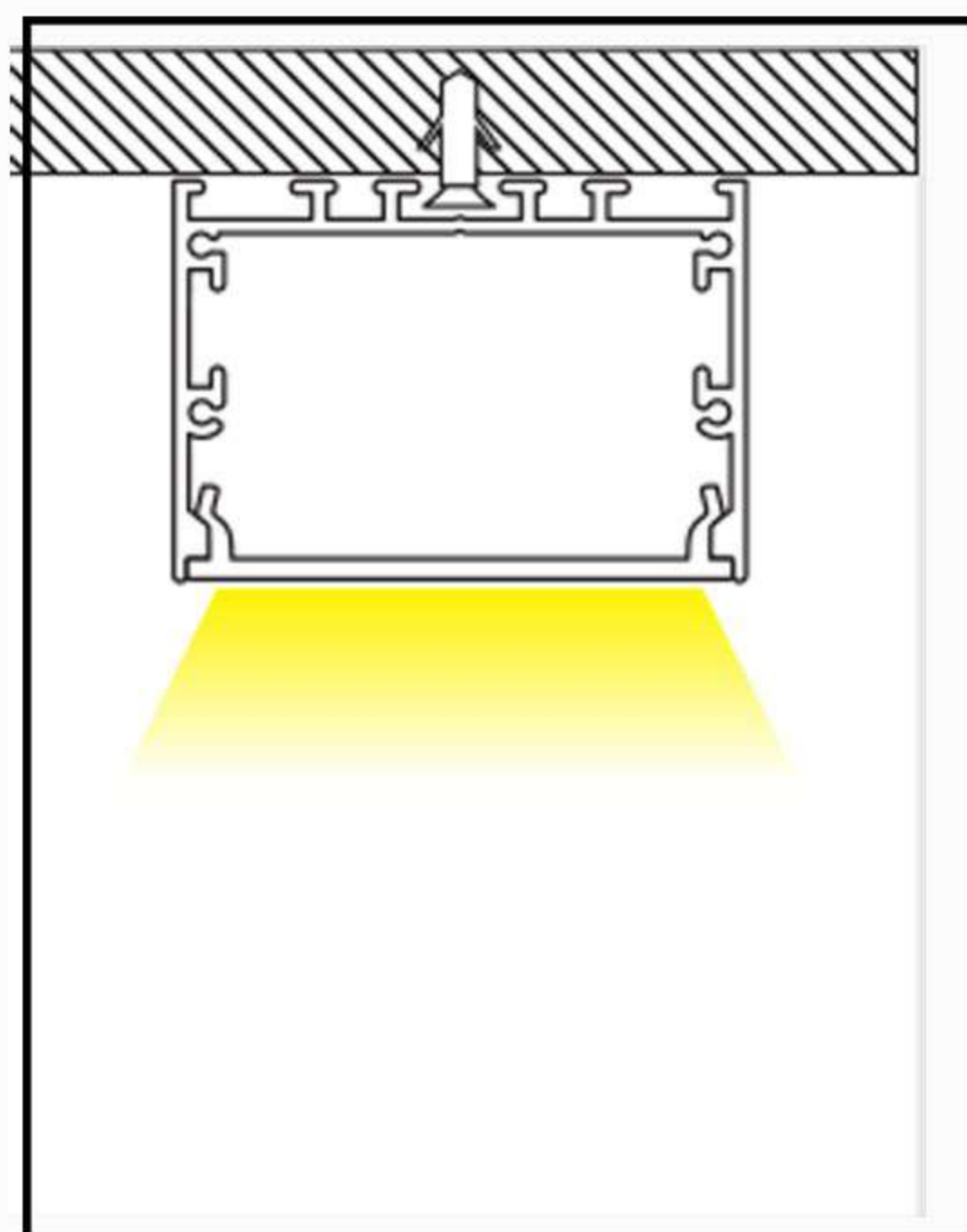
Ceiling Mount
