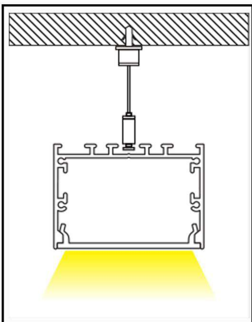
Hanging Installation
