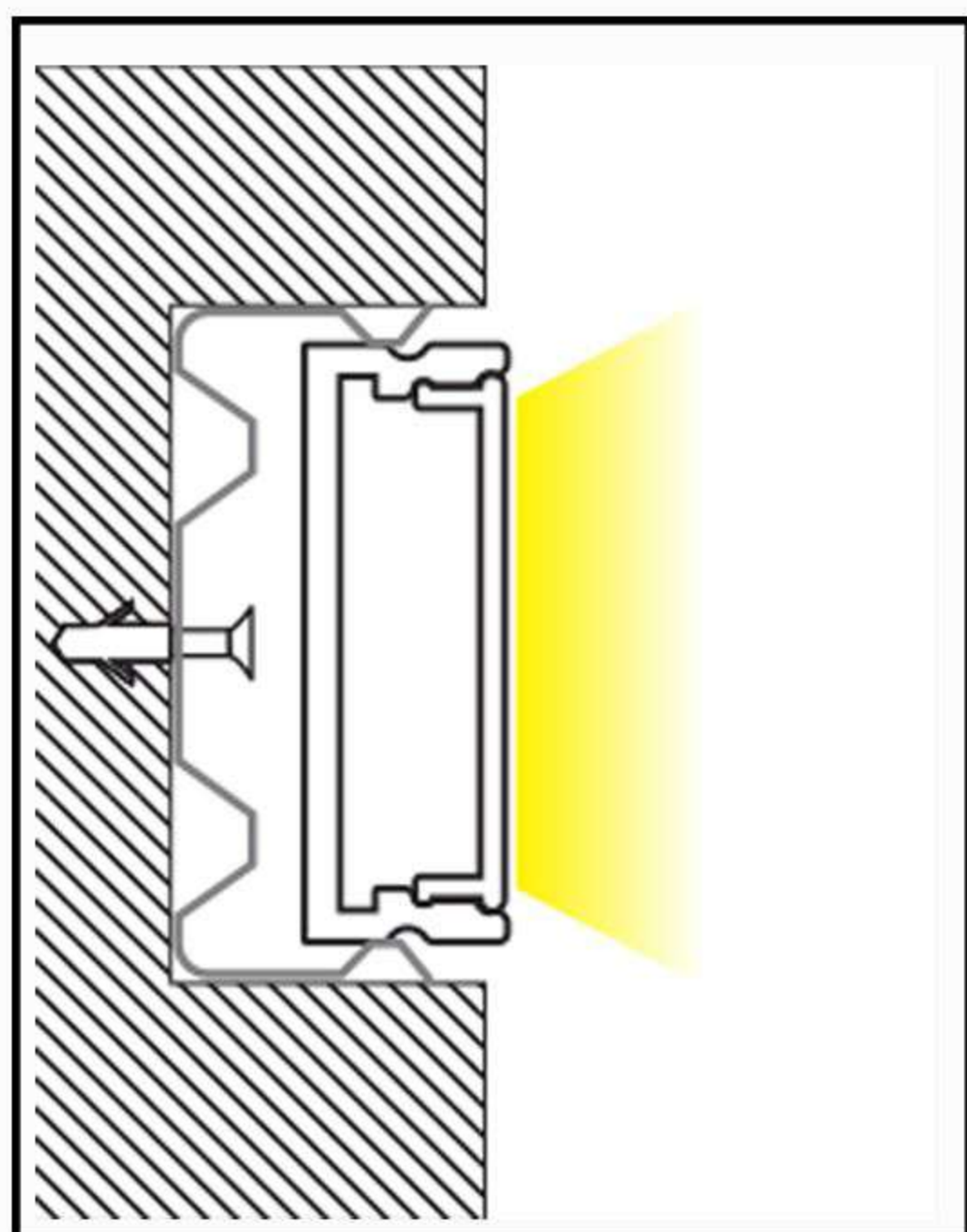
Embedded Installation
